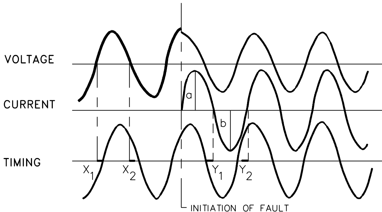
Figure 3 Determination of current and power factor for circuits of 10,000 amperes and less (See Clause 5.17.3.2.1)
