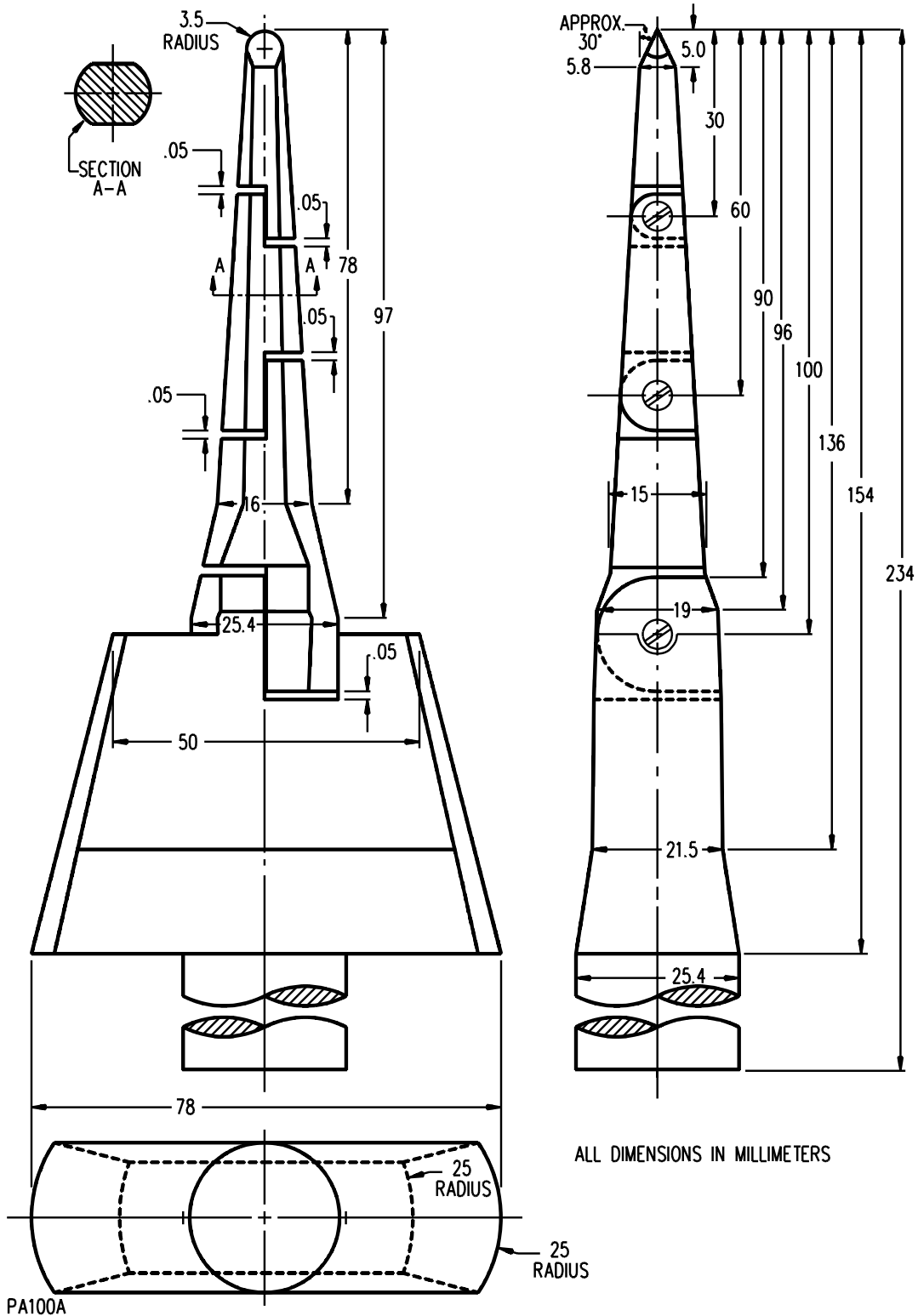
Figure 1 Articulate probe with web stop
