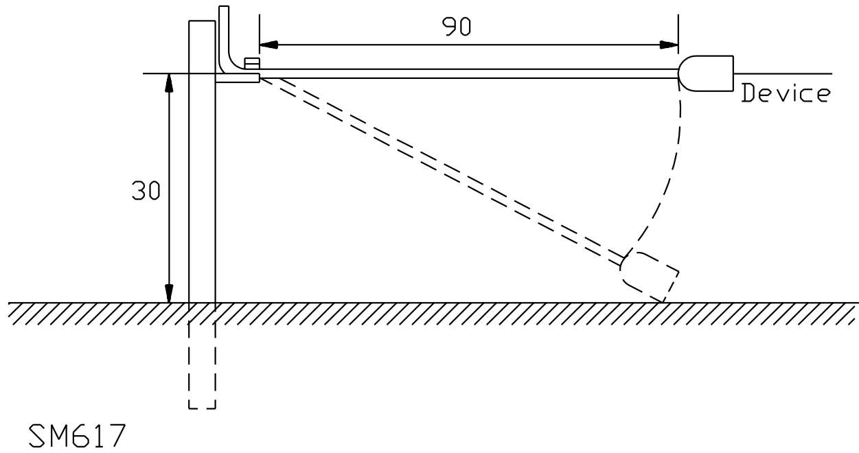
Figure 2 Impact test equipment (See Clause 5.13.2)
